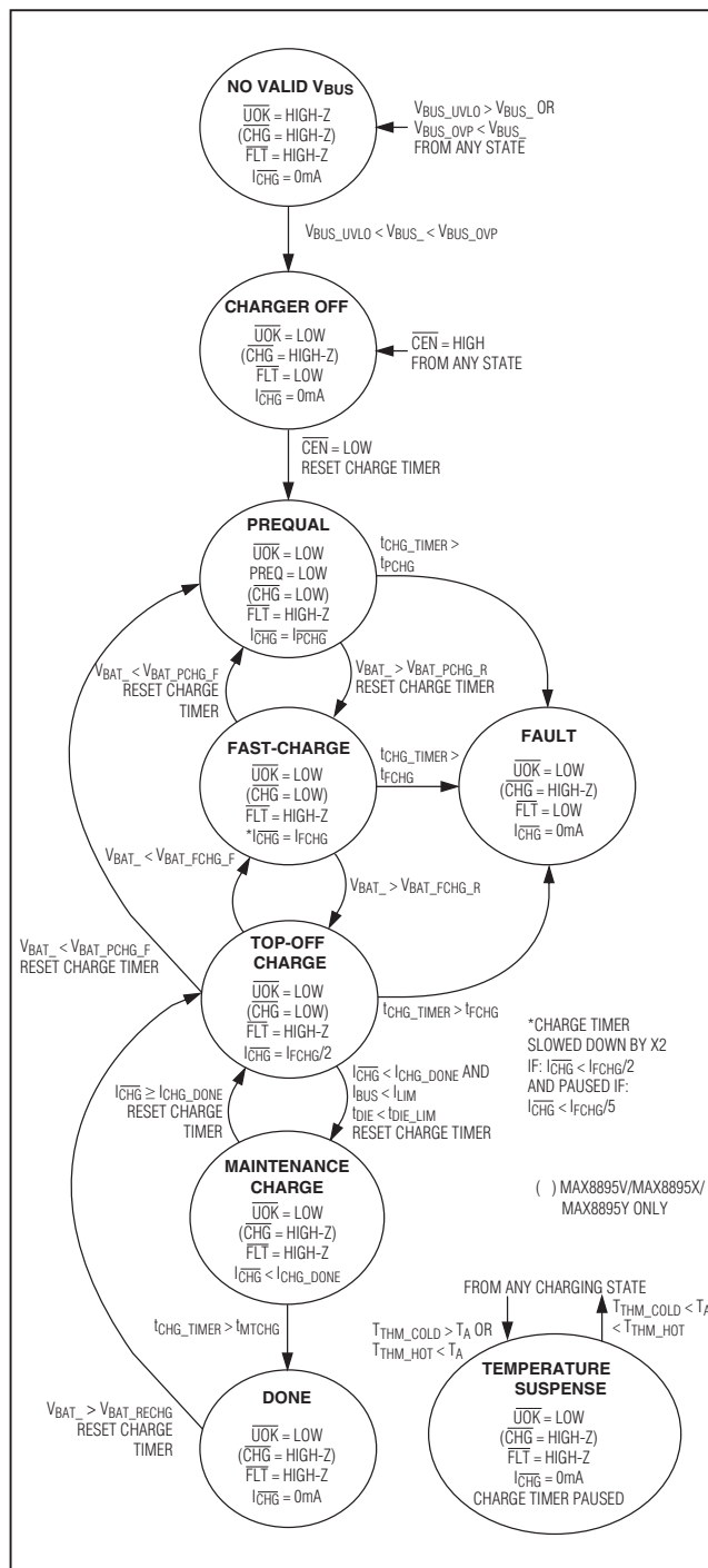
Figure 23. Charger Flow Chart
