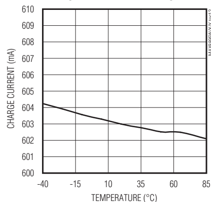
CHARGE CURRENT (DEDICATED CHARGER) vs. AMBIENT TEMPERATURE
