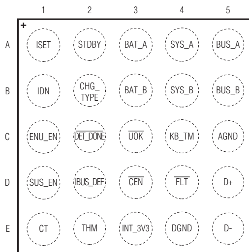
TOP VIEW (BUMP SIDE DOWN)
