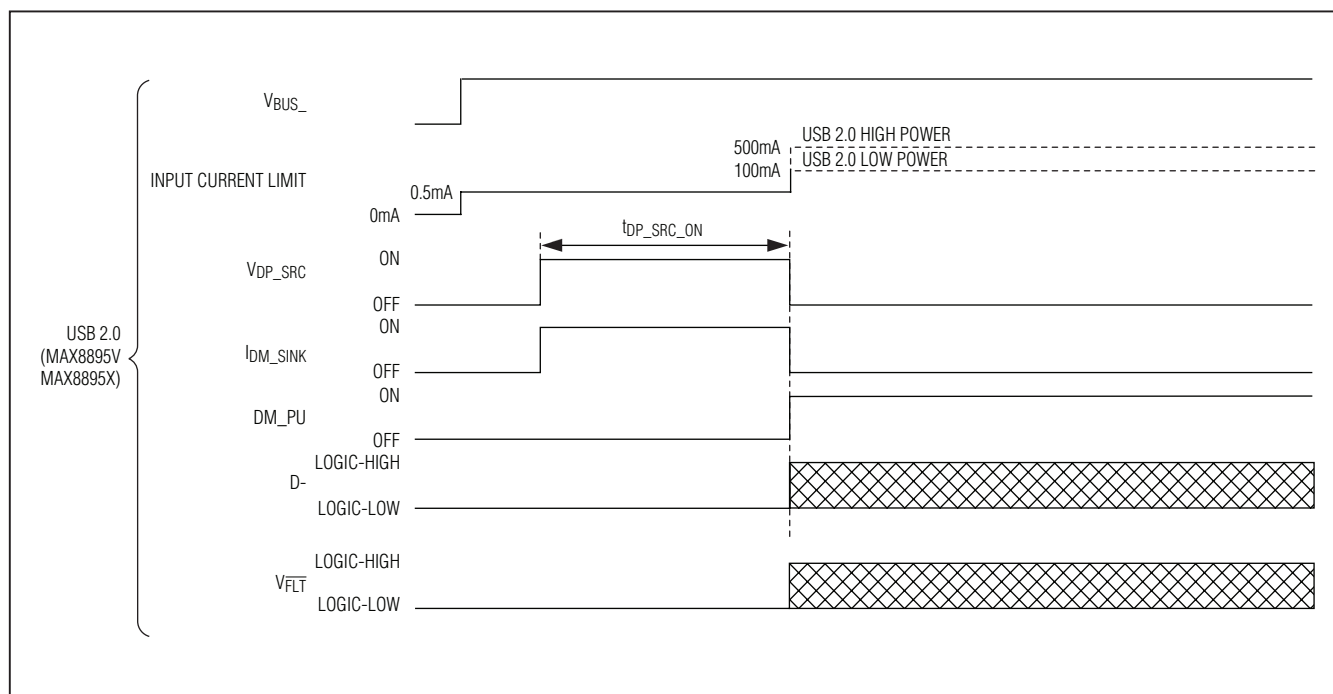
Figure 14b. USB Detection Timing Diagram (MAX8895V/MAX8895X)
