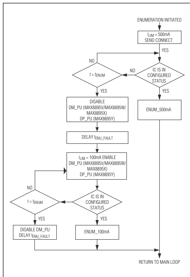
Figure 13. Flow Chart for Enumeration Process
