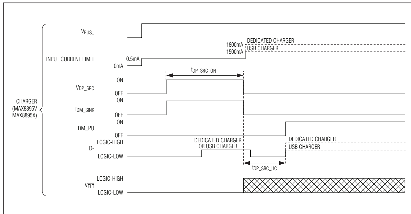
Figure 14a. Charger Detection Timing Diagram (MAX8895V/MAX8895X)
