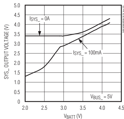
SYS_ OUTPUT VOLTAGE vs. BATTERY VOLTAGE
