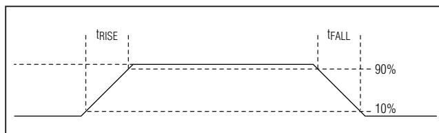
Figure 7. USB Rise and Fall Timing
