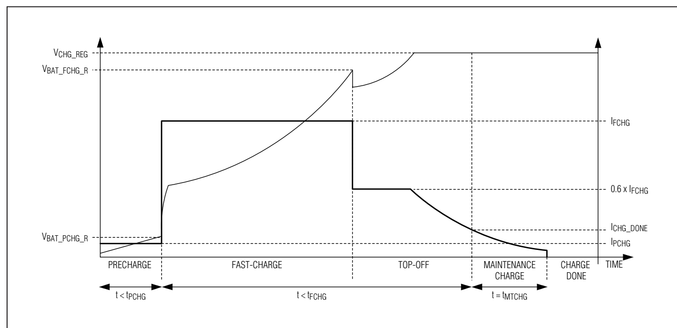
Figure 22. Charging States
