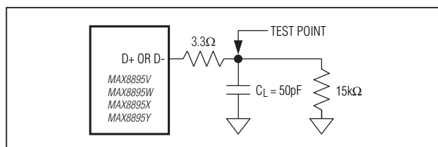
Figure 8. Load for D+/D- AC Measurements
